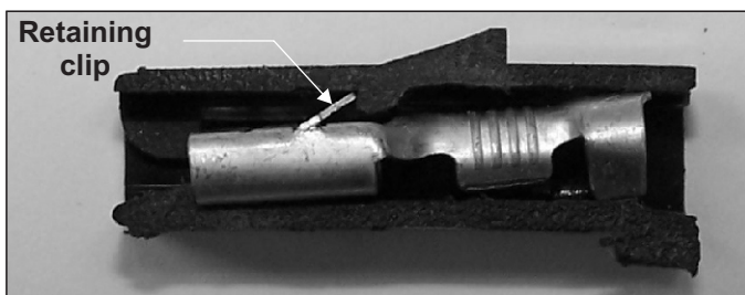
To release the terminal, depress the retaining clip and pull the terminal out from the wire end.
