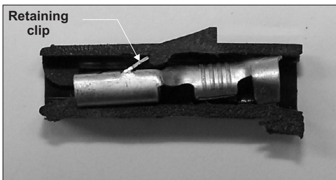
To release the terminal, depress the retaining clip and pull the terminal out from the wire end.
